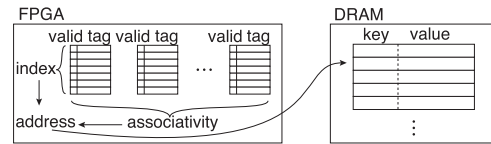
Fig. 11 Correspondence of the hash table and the value storage.
