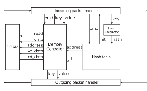
Fig. 10 NIC cache architecture.
