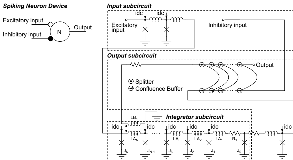
Fig. 2. Spiking neuron device consisting of SFQ circuits.
