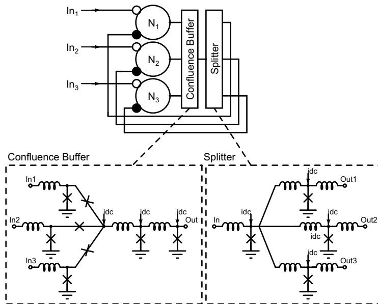
Fig. 3. Inhibitory neural network consisting of three spiking neurons, a 3-input confluence buffer, and a 3-output splitter.
