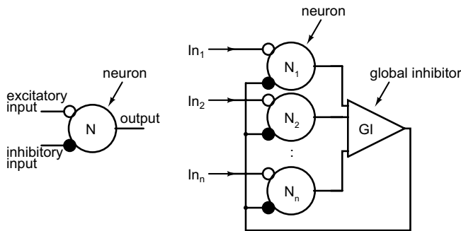
Fig. 1. Inhibitory neural network consisting of a number of neurons and a global inhibitor.
