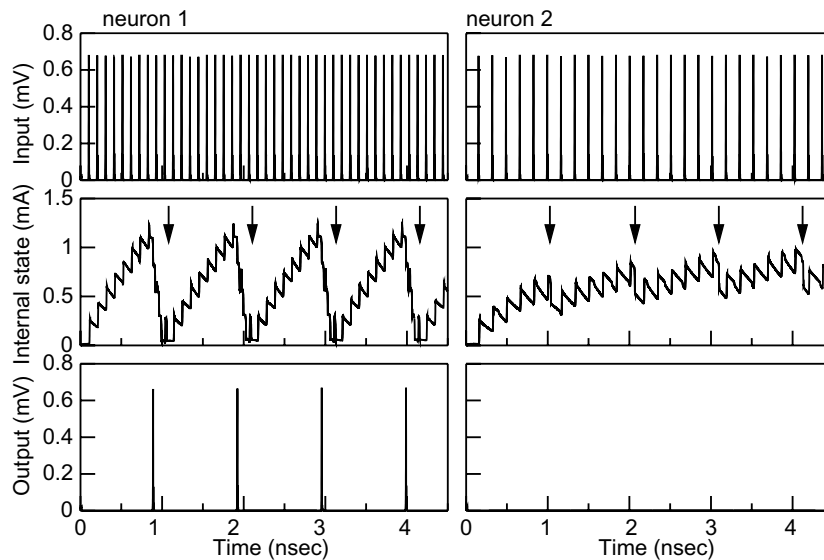
Fig. 4. Operation of the spiking neural network. Simulated results of (i) input pulses, (ii) internal state, and (iii) output pulse, for neuron N_1 and N_2 .
